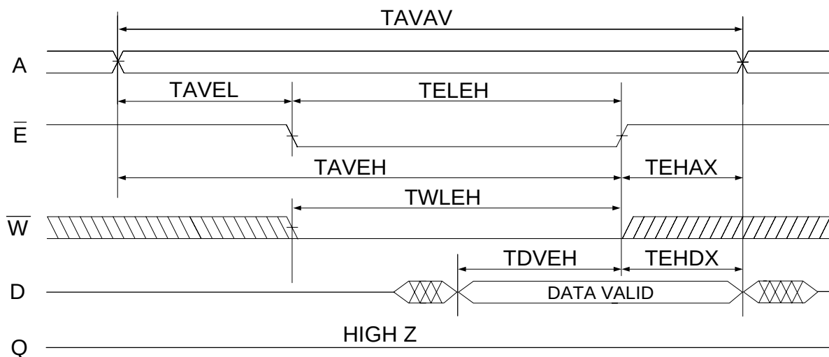
WRITE CYCLE 2 - \overline{E} CONTROLLED
