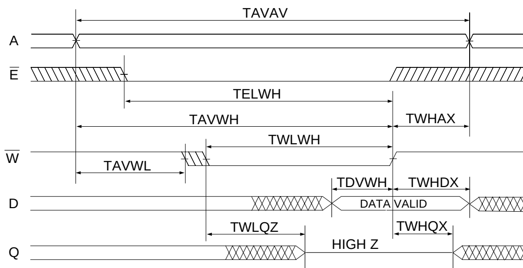
WRITE CYCLE 1 - \overline{W} CONTROLLED
