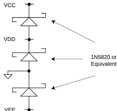
Figure 1. Power Supply Protection Scheme
