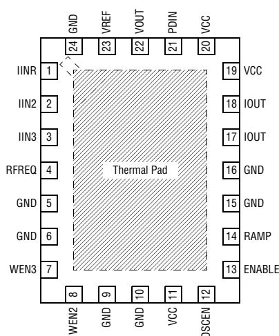
24-Pin LPP Top View
