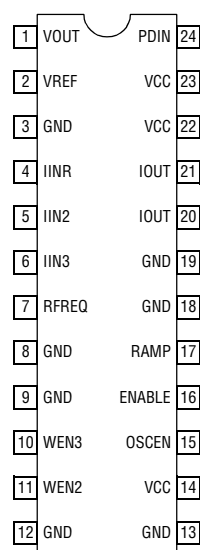
24-Pin QSOP
