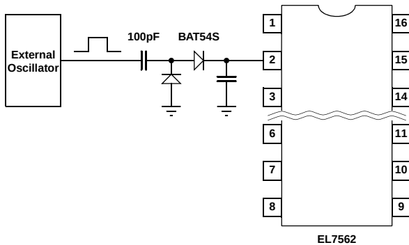
FIGURE 1. OSCILLATOR SYNCHRONIZATION
