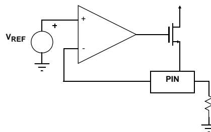
FIGURE 1. R_{FREQ} PIN INTERFACE
