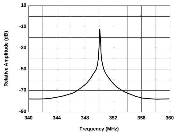
Output Spectrum-Wideband
