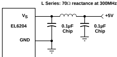
FIGURE 2. RECOMMENDED SUPPLY BYPASSING
