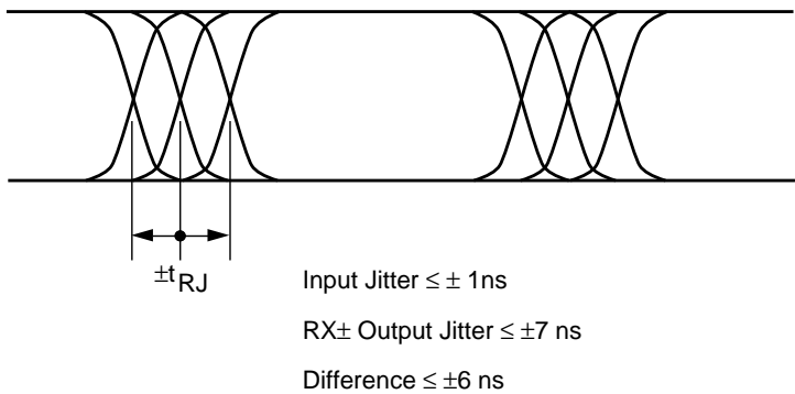
Figure 8. Receive Jitter Timing
