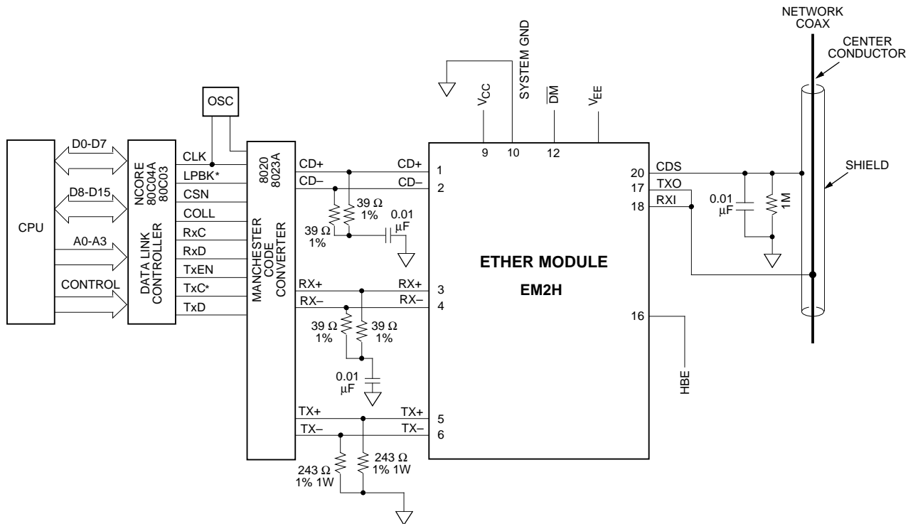
Figure 5a. Coax Ethernet Transceiver System Connections
