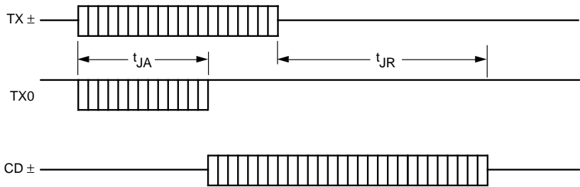
Figure 7. Jabber Timing
