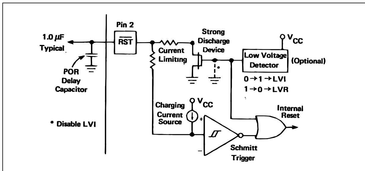
Figure 14 : RESET Configuration.
