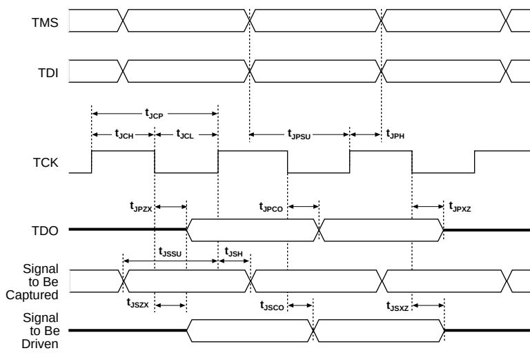
Figure 9. EPC2 JTAG Waveforms
