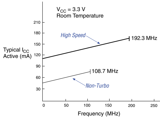
Figure 13. I_{CC} vs. Frequency for MAX 3000A Devices
