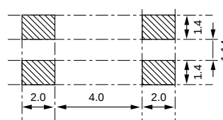
Figure 6) CSM-8B – Recommended Solder Pad Layout Top view
