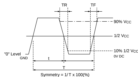
Figure 4) Output Wave Form
