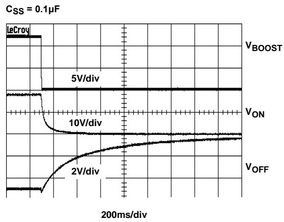
FIGURE 27. POWER-DOWN, 100k AND 0.1 \mu F DELAY NETWORK ON ENP
