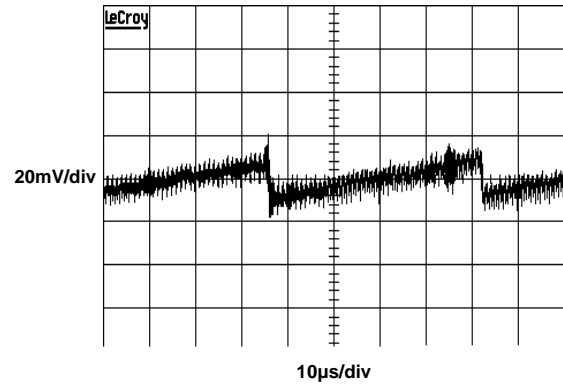
FIGURE 20. V_{OFF} RIPPLE
