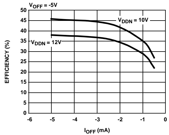
FIGURE 10. EFFICIENCY vs I_{OFF}
