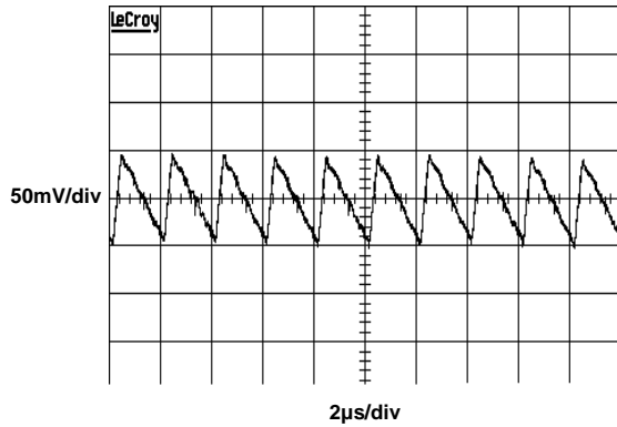
FIGURE 19. V_{ON} RIPPLE
