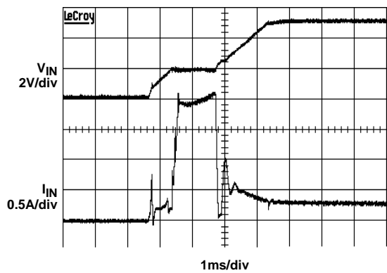
FIGURE 23. START-UP VOLTAGE AND CURRENT
