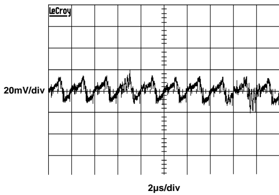
FIGURE 21. V_{OFF} RIPPLE
