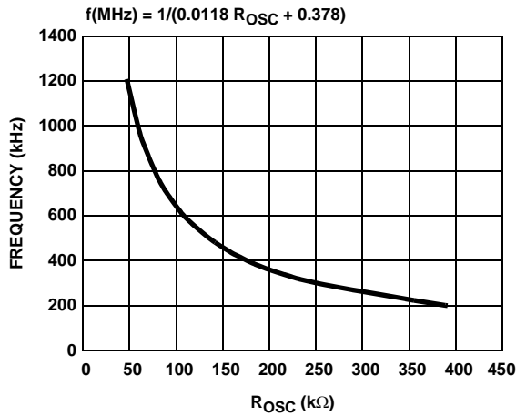
FIGURE 13. F_S vs R_{\text{OSC}}
