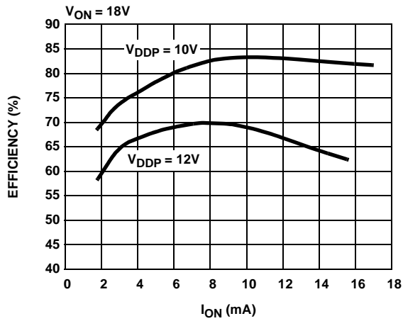
FIGURE 9. EFFICIENCY vs I_{ON}
