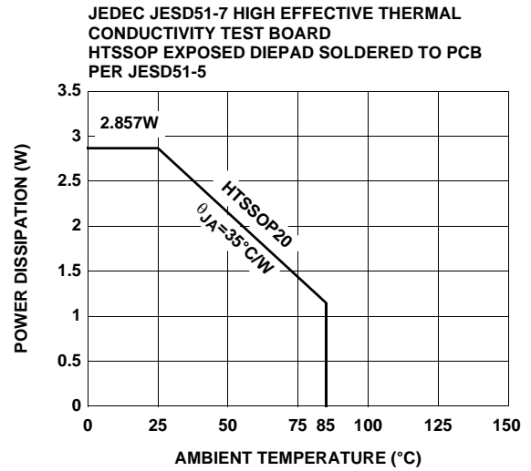
FIGURE 32. PACKAGE POWER DISSIPATION vs AMBIENT TEMPERATURE
