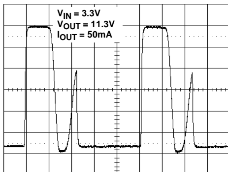
FIGURE 29. LX WAVEFORM - DISCONTINUOUS MODE
