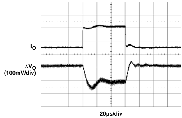
FIGURE 22. BOOST CONVERTER TRANSIENT RESPONSE
