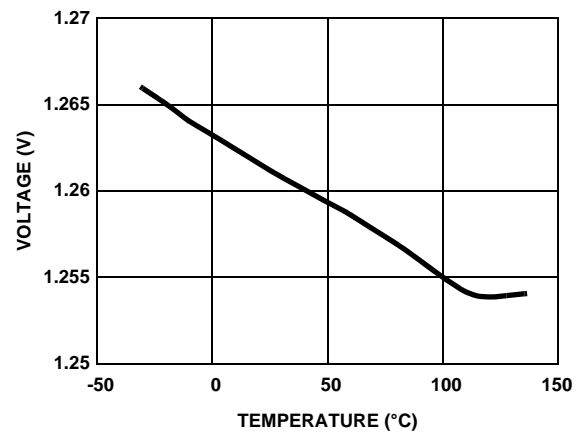
FIGURE 16. V_{\text{REF}} vs TEMPERATURE
