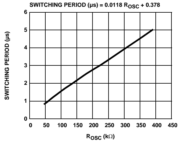
FIGURE 14. SWITCHING PERIOD vs R_{\text{OSC}}
