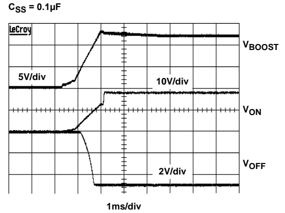
FIGURE 28. POWER-UP, 100k AND 0.1 \mu F DELAY NETWORK ON ENP
