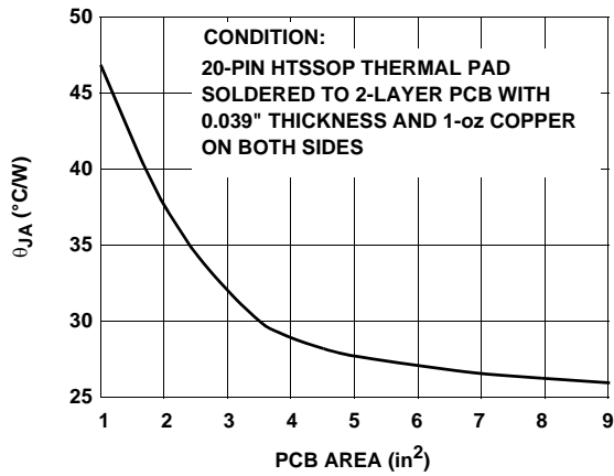
FIGURE 31. 20-PIN HTSSOP THERMAL RESISTANCE vs PCB AREA, NO AIR FLOW
