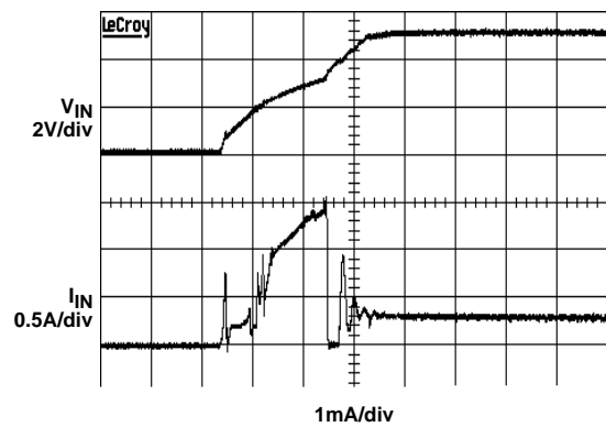
FIGURE 24. START-UP VOLTAGE AND CURRENT
