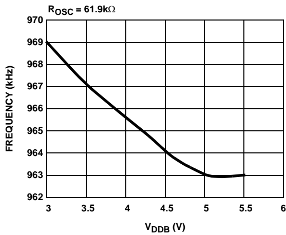
FIGURE 15. F_S vs V_{\text{DDB}}
