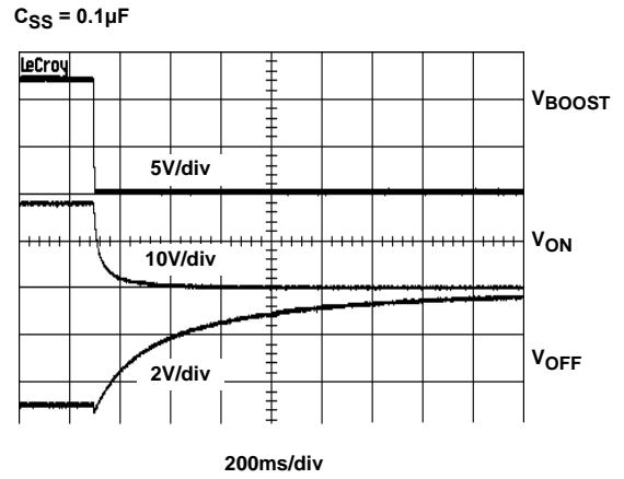
FIGURE 26. POWER-DOWN, NO DELAY RC NETWORK ON ENABLE PINS
