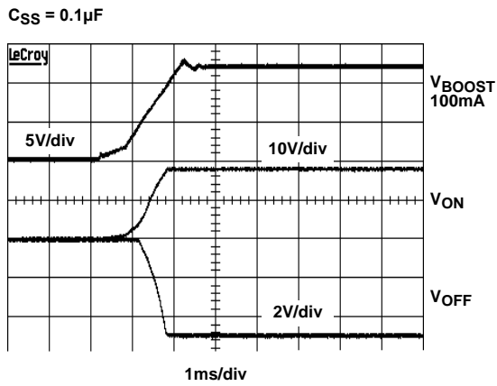
FIGURE 25. POWER-UP, NO DELAY RC NETWORK ON ENABLE PINS
