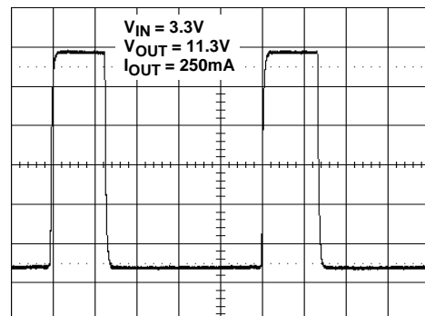
FIGURE 30. LX WAVEFORM - CONTINUOUS MODE
