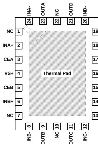
EL5492A (24-PIN LPP) TOP VIEW
