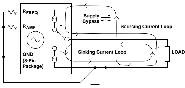
FIGURE 2. OUTPUT CURRENT LOOPS
