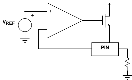
FIGURE 3. R_{FREQ} AND R_{AMP} PIN INTERFACE
