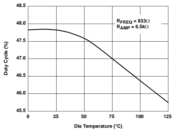
Duty Cycle vs Die Temperature
