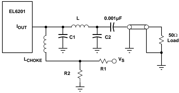
FIGURE 4. TUNED INTERFACE TO 50Ω LEAD
