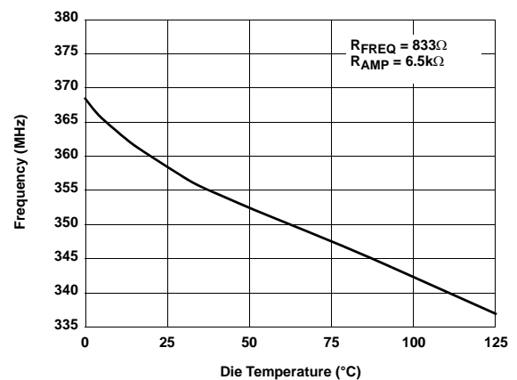
Frequency vs Die Temperature
