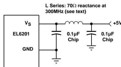
FIGURE 1. RECOMMENDED SUPPLY BYPASSING
