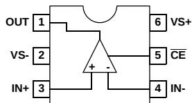
EL5193A (6-PIN SOT-23) TOP VIEW
