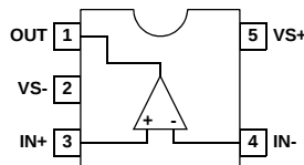
EL5193 (5-PIN SOT-23) TOP VIEW
