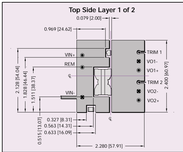
Figure 19a - Recommended Top Side Footprint
