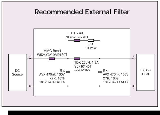
Figure 9 - Recommended External Input Filter
