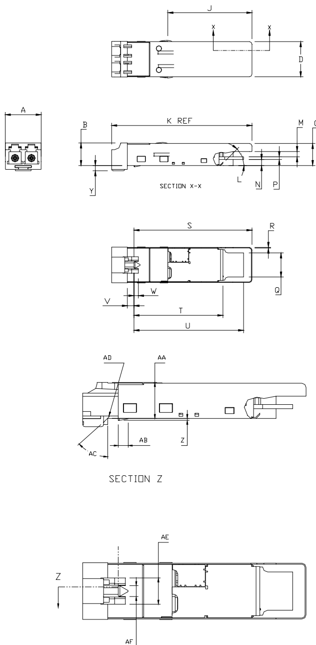
Figure 1: SFP Transceiver Package Dimensions (-MS Version shown)
