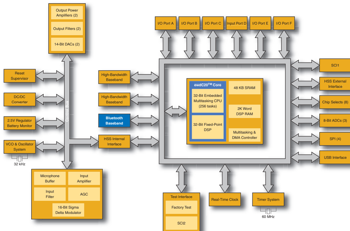
e8720 Wireless Processor Block Diagram
