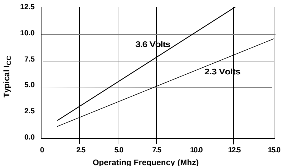
FIGURE 2: Typical Operating Current Curves
