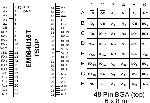
FIGURE 1: Pin Configurations
