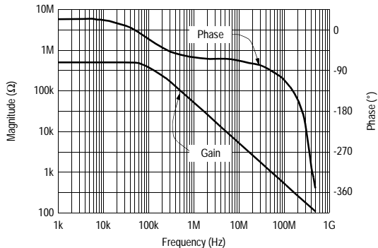
Transimpedance (ROL) vs Frequency
