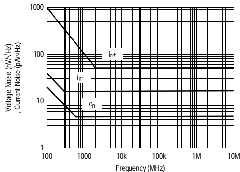
Voltage and Current Noise vs Frequency
