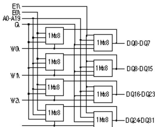
EDI7F2331MC-BNC 2x1Megx32 80 pin SIMM
