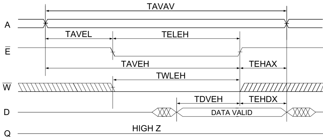
FIG. 5 WRITE CYCLE 2 - E CONTROLLED
