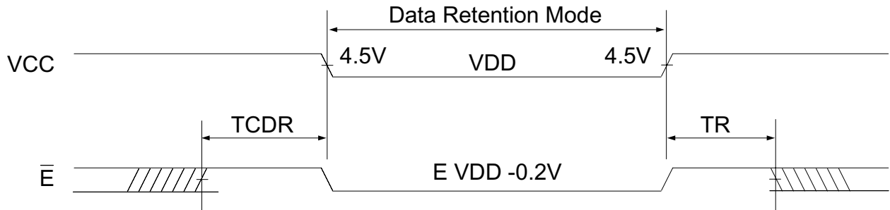
FIG. 6 DATA RETENTION - E CONTROLLED
