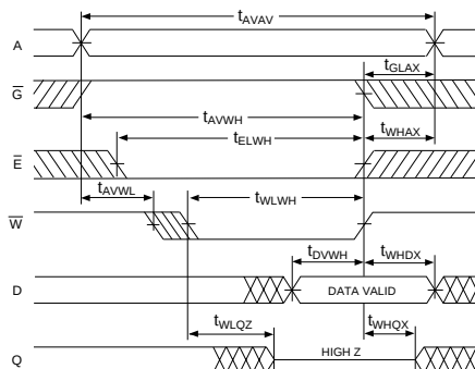
FIG. 6 WRITE CYCLE 1 - \overline{W} CONTROLLED
