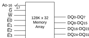
BLOCK DIAGRAM
