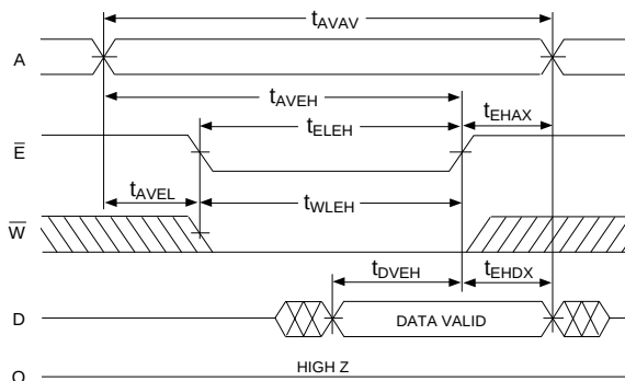
FIG. 7 WRITE CYCLE 2 - \overline{E} CONTROLLED
