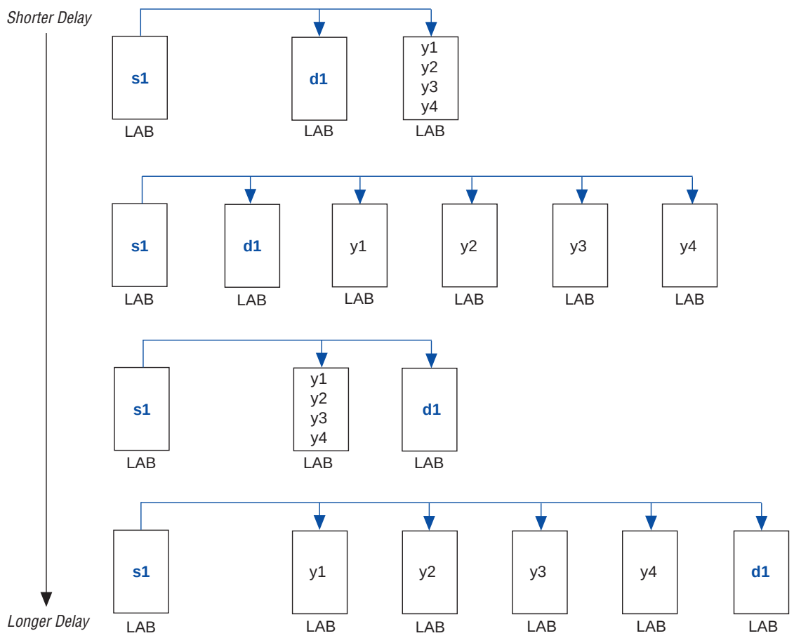
Figure 12. Delay from s1 to d1 as a Function of Relative Position & Load Distribution
