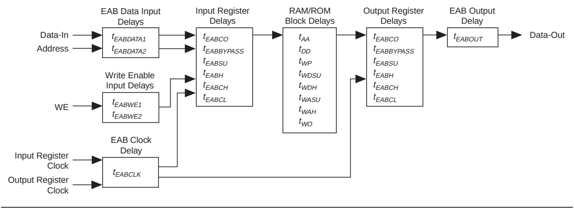
Figure 8. FLEX 10K Device EAB Timing Model
