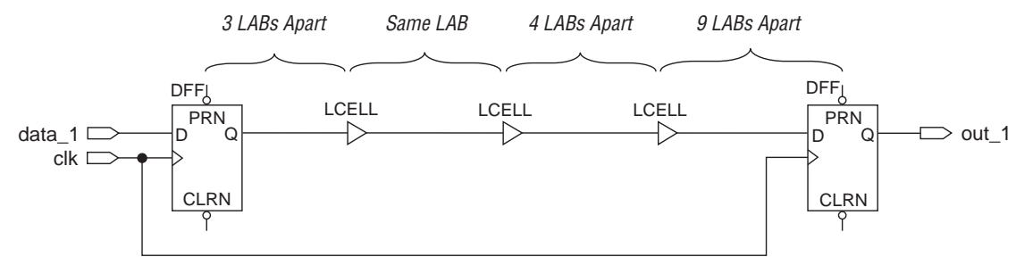
Figure 1. Path for t_{\text{DDR}} Circuit for 21-Column FLEX 8000 Devices
