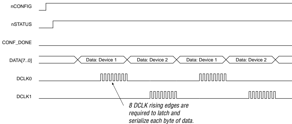
Figure 7. Multi-Device Passive Parallel Synchronous (MD-PPS) Configuration Waveforms
