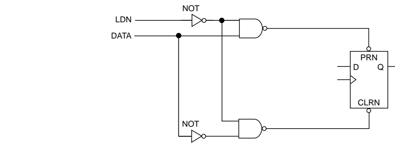
Figure 3. Asynchronous Load without a Clear Input Signal
