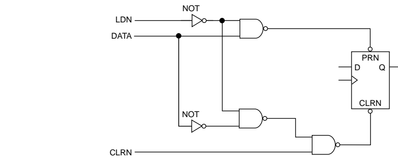
Figure 2. Asynchronous Load with a Clear Input Signal
