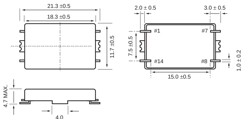
ECX-TXO-10C2 SERIES – Top, Side and Bottom views
