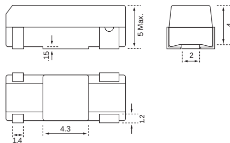
Figure 1) ECX-3A - Top, Side, Bottom and End views
