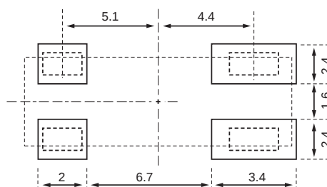
Figure 2) ECX-3A Land Pattern - Bottom view
