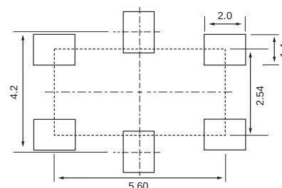
Figure 3) ECS-96SMF Land Pattern
