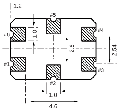
Figure 2) ECS-96SMF Pad Layout - Bottom view
