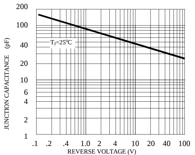
FIG. 6-TYPICAL JUNCTION CAPACITANCE
