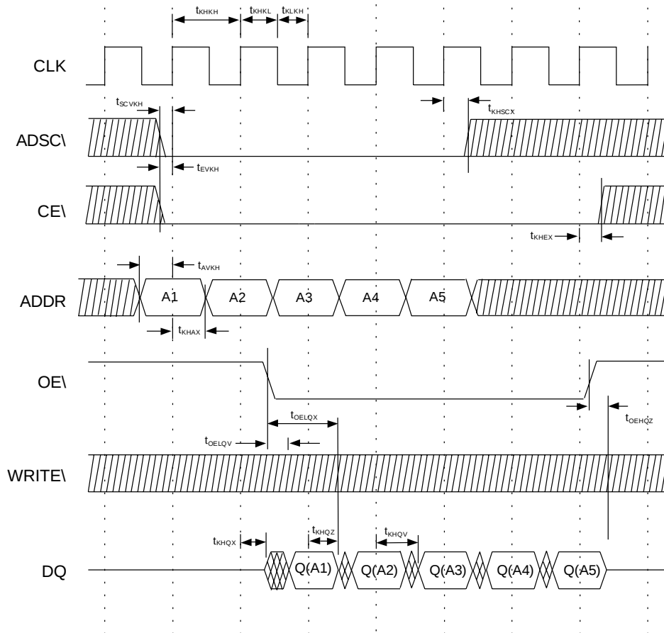
FIG. 2 READ TIMING
