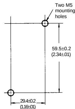
Mounting holes
