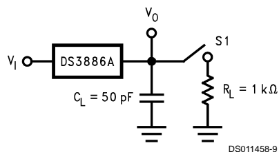
FIGURE 4. Driver: ACLK to Bn, t_s , t_H , t_{PW}
