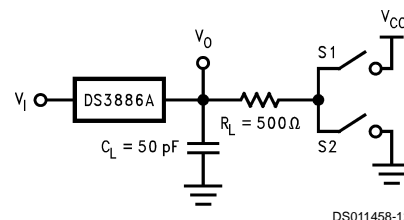
FIGURE 7. Receiver Enable/Disable Set-up
