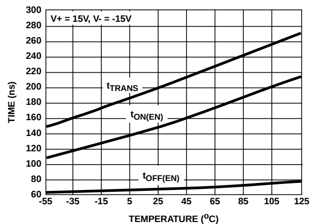
FIGURE 13. t_{ON}/t_{OFF} vs TEMPERATURE
