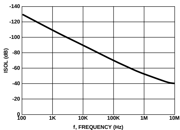
FIGURE 11. OFF ISOLATION vs FREQUENCY
