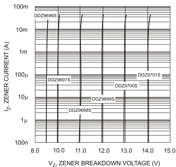
Fig. 5 Typical Reverse Characteristics, DDZ9696S - DDZ9701S
