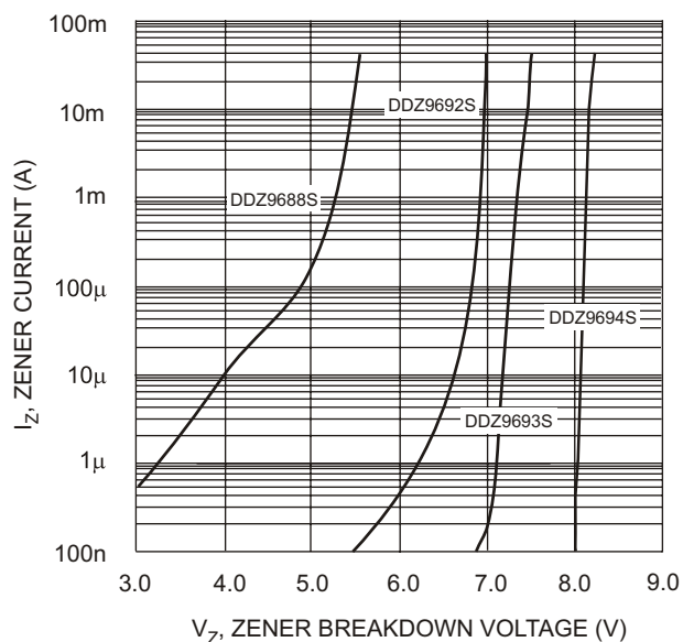
Fig. 4 Typical Reverse Characteristics, DDZ9688S - DDZ9694S
