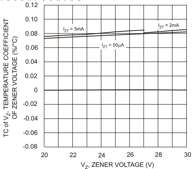
Fig. 18 Typical Temperature Coefficient of Zener Voltage, DDZ9707 - DDZ9713
