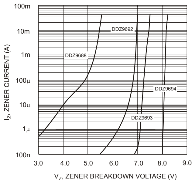
Fig. 4 Typical Reverse Characteristics, DDZ9688 - DDZ9694
