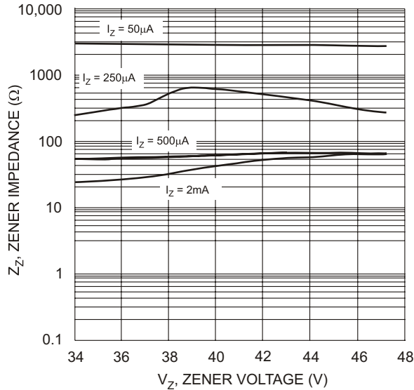
Fig. 14 Typical Zener Impedance Characteristics, DDZ36S - DDZ47S
