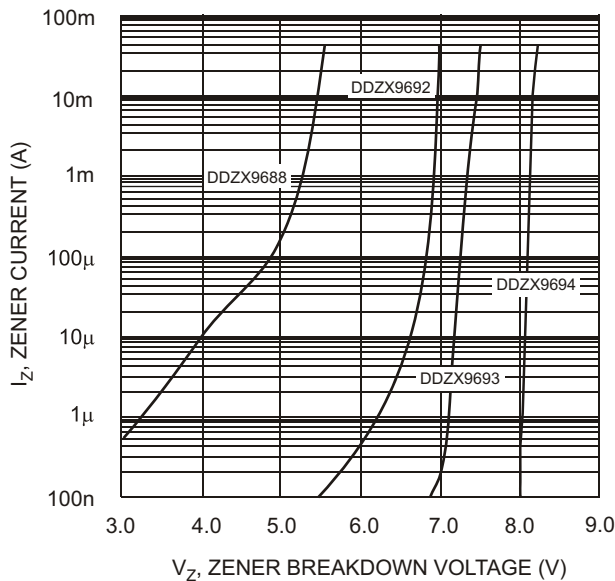
Fig. 4 Typical Reverse Characteristics, DDZX9688 - DDZX9694
