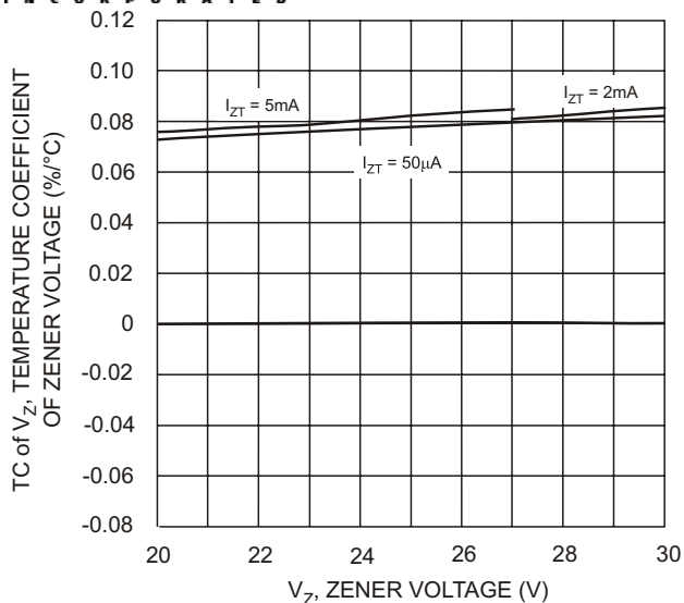
Fig. 18 Typical Temperature Coefficient of Zener Voltage, DDZX9707 - DDZX9713
