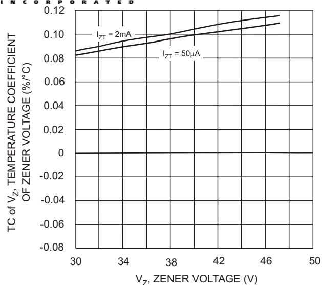
Fig. 18 Typical Temperature Coefficient of Zener Voltage, DDZX30DTS-DDZX47TS
