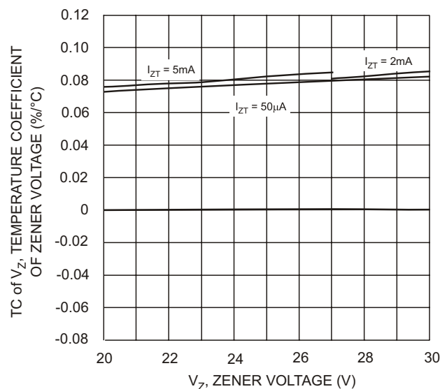
Fig. 17 Typical Temperature Coefficient of Zener Voltage, DDZX20CTS-DDZX30DTS
