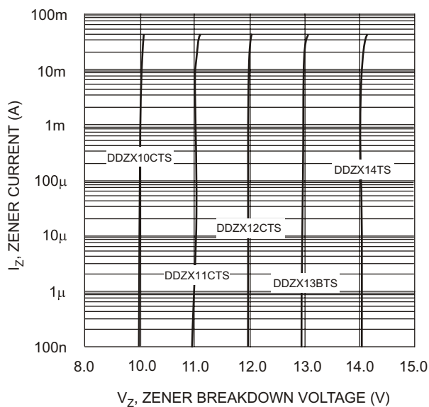
Fig. 5 Typical Reverse Characteristics, DDZX10CTS - DDZX14TS
