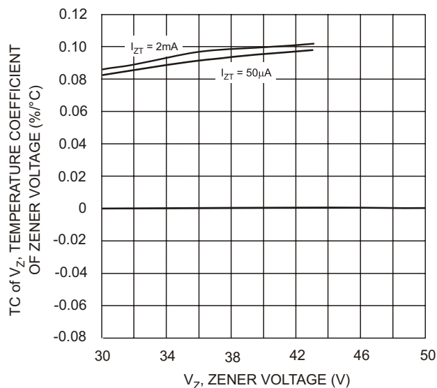
Fig. 18 Typical Temperature Coefficient of Zener Voltage, DDZX30D-DDZX43
