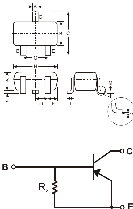
SCHEMATIC DIAGRAM
