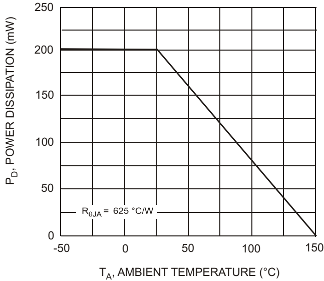
Fig. 1, Derating Curve
