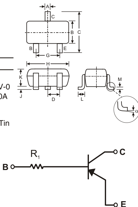
SCHEMATIC DIAGRAM
