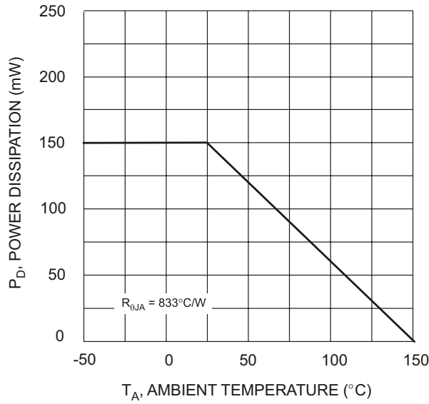
Fig. 1 Derating Curve
