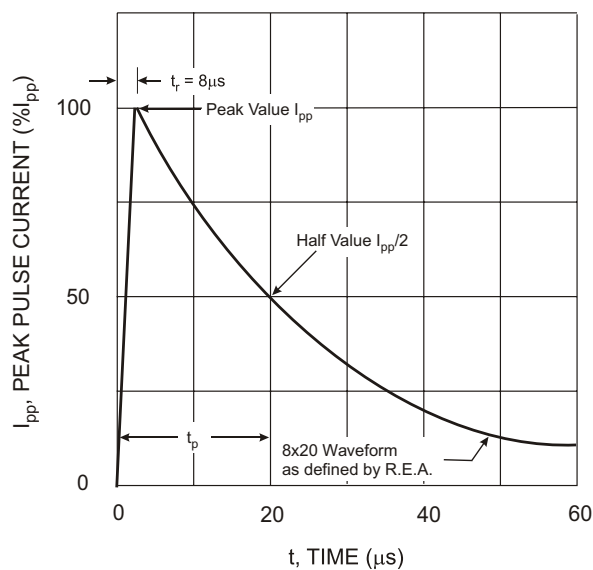
Fig. 4 Pulse Waveform
