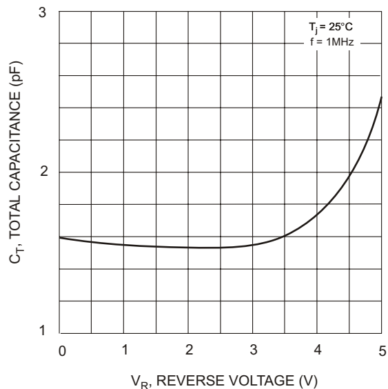
Fig. 2 Typ. Total Capacitance vs Reverse Voltage
