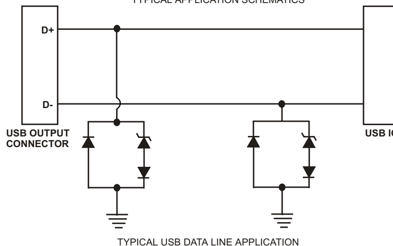
TYPICAL APPLICATION SCHEMATICS
