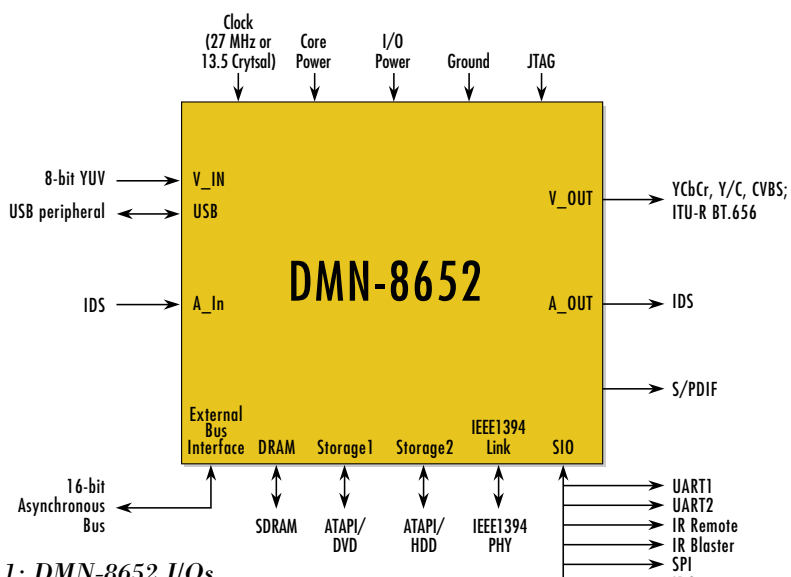
Figure 1: DMN-8652 I/Os
