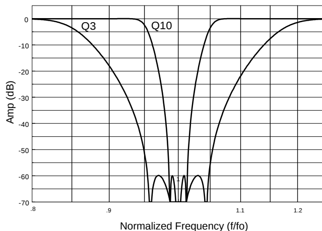
Normalized Theoretical Amplitude Data
