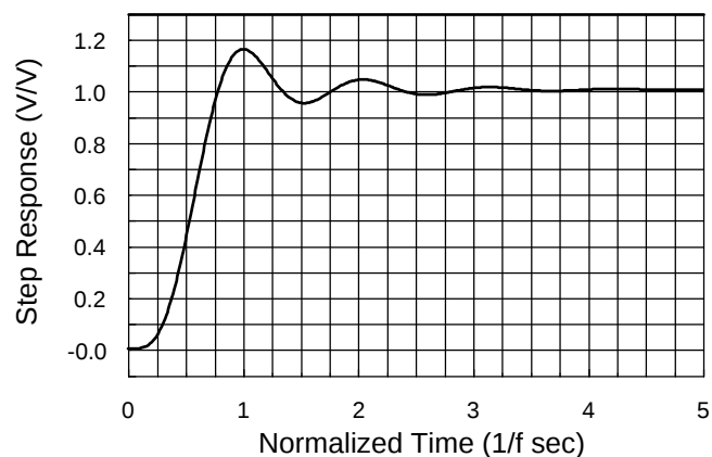
Step Response
