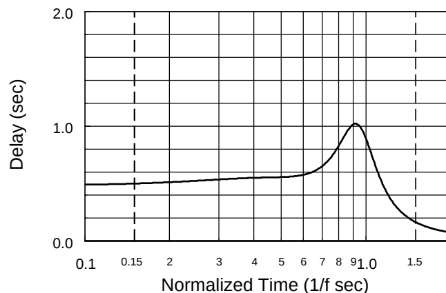
Delay (Normalized)
